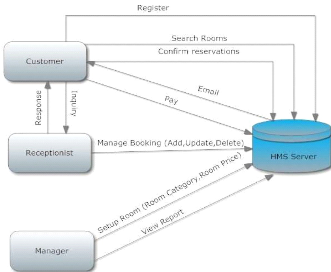
Figure 2.2 System Architecture
